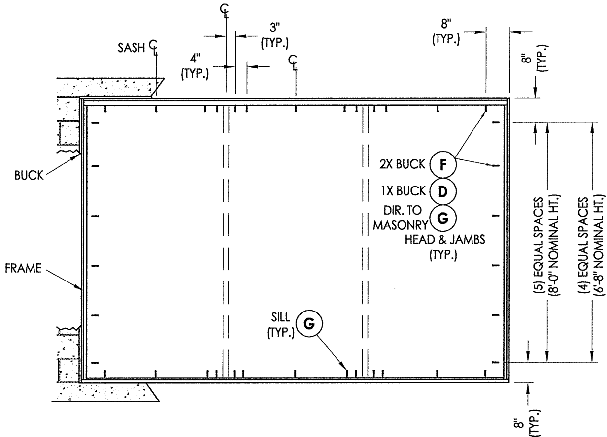
FRAME ANCHORING
